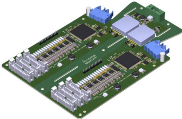
Dual Channel Gate Drive
